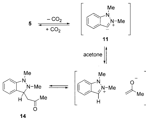
Scheme 7. Formal CH-insertion into the methyl group of acetone by the nucleophilic carbene.
