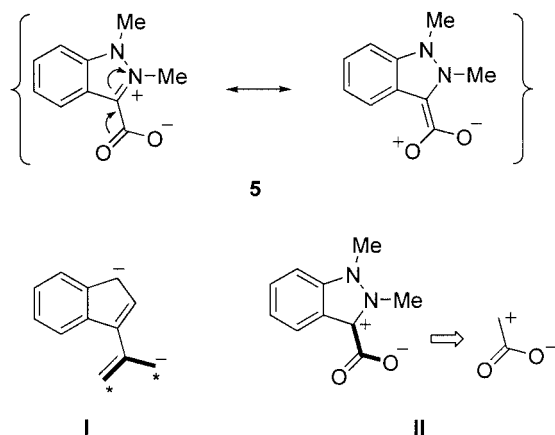
Scheme 3. Characteristic features of pseudo-cross-conjugation.
