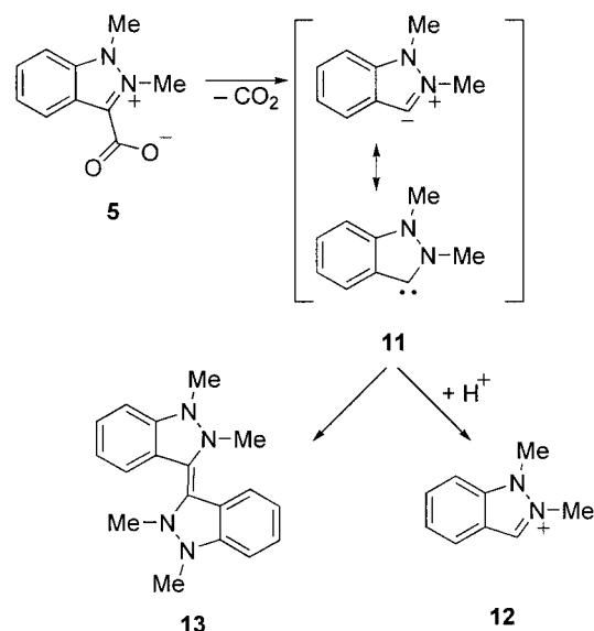
Scheme 6. Decarboxylation produces a nucleophilic carbene 11 and characteristic trapping products.
