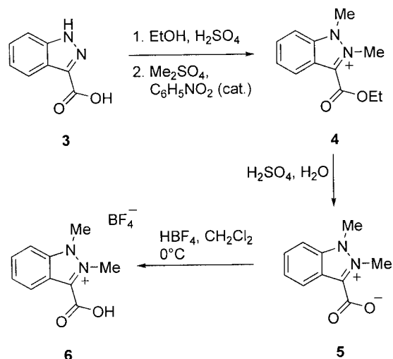
Scheme 2. Synthesis of indazolium-3-carboxylate 5 as model compound for the pseudo-cross-conjugated mesomeric betaine alkaloid Nigellidine.
