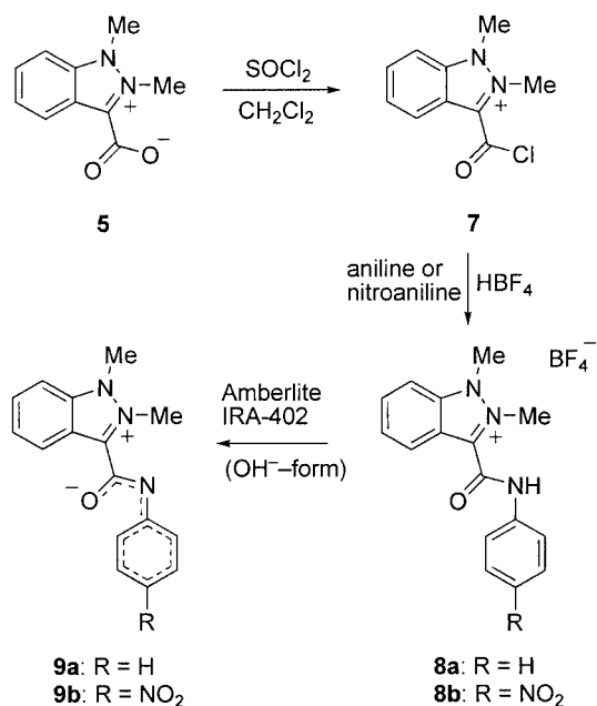
Scheme 4. Synthesis of new PCCMBs: amidates.
