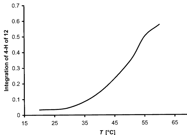
Figure 1. Decarboxylation of the mesomeric betaine 5 in [\text{D}_6] -DMSO with temperature; Integration of the signal of 4-H of the resulting indazolium salt 12 .
